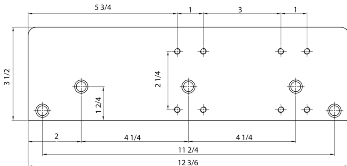
GFDB440 Drop plate (Regular arm mount)
