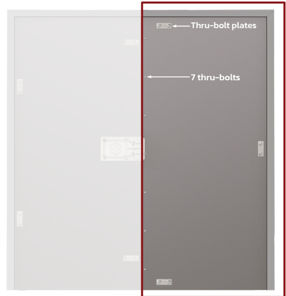
Inactive leaf
