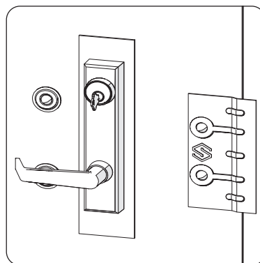
Trim for self-locking Tridents, on individual trim plate
