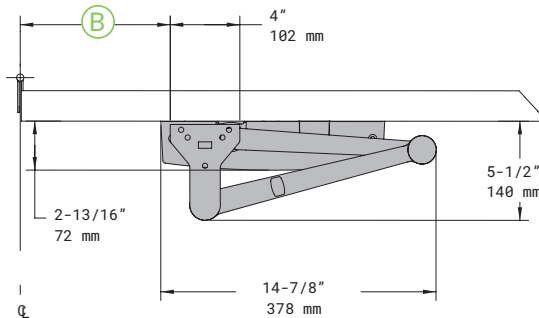
EDA Mount
