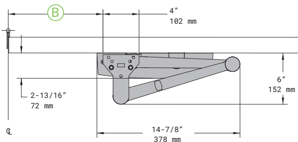
CUSH Mount
