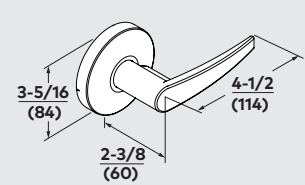
LG Lever
