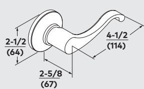
LS Lever
