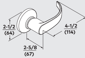
L118 Lever
