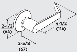
LR Lever
