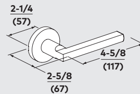
L118 Lever
